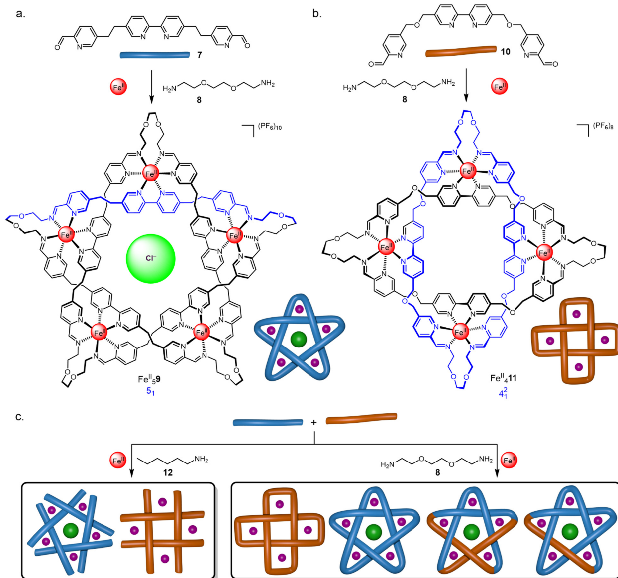
Fig. 5 Self-assembly of (a) molecular pentafoil knot 43 Fe 5 II 9 and (b) Solomon link 45 Fe 4 II 11 using dynamic imine exchange. (c) Self-sorting of circular helicates, knots and links. 46
