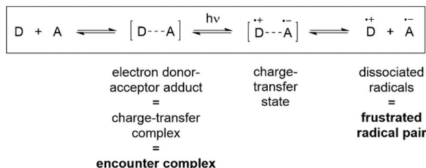
Fig. 6 Mulliken theory for electron transfer in electron donor–acceptor adducts, with analogous terms relevant to FLP chemistry highlighted in bold.
