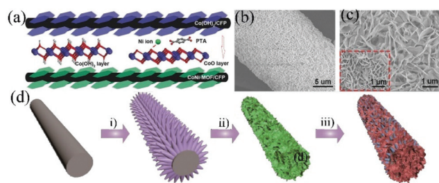
Fig. 2 (a) The schematic illustration of the synthesis of CoNi-MOF, and the SEM images of (b) the \text{Co(OH)}_2 precursor and (c) CoNi-MOF. Reprinted with permission from ref. 51, Copyright 2017, Wiley-VCH. (d) Schematic illustration of the preparation of CC/CoNi-MOF. (i) Formation of ZnO nanoarrays, (ii) deposition of \text{Co(OH)}_2 nanosheets and (iii) transformation of \text{Co(OH)}_2 to CoNi-MOF. Reprinted with permission from ref. 53, Copyright 2020, Elsevier.
