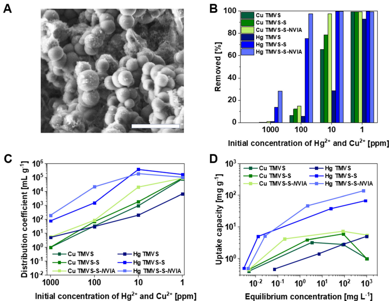
Fig. 2 (A) SEM image of TMVS-S-NVIA particles. Scalebar is 5 \mu m. (B) Removed copper ions (green) and mercury ions (blue) from aqueous solution by TMVS-S and TMVS-S-NVIA particles in %. Calculated distribution coefficients (C) and uptake capacities (D) of TMVS-S particles and TMVS-S-NVIA particles, respectively. Uptake capacities plotted against initial ion concentration can be found in the ESI.†
