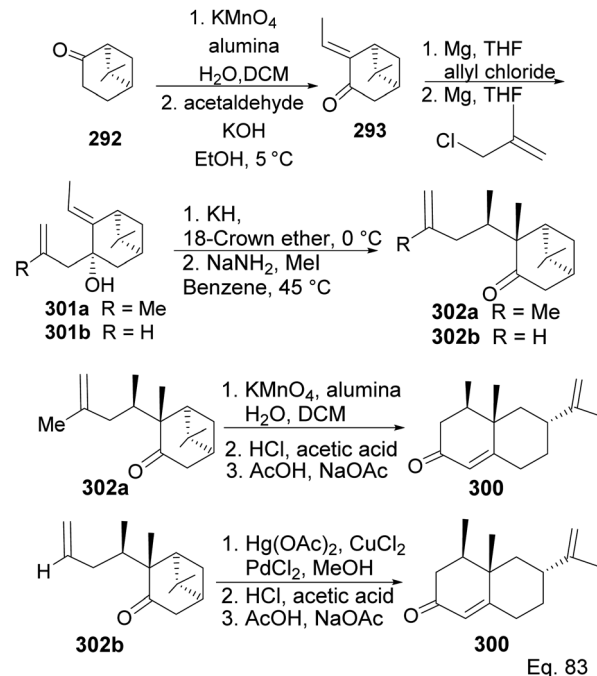
Scheme 77 Synthesis of (+)-nootkatone from nopinone via stereospecific oxy-Cope rearrangement of ( E )-3-allyl-2-ethylidene-6,6-dimethylbicyclo[3.1.1]heptan-3-ol ( 301 ).
