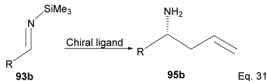
Scheme 27 \text{Ip}^2\text{B}(\text{allyl})\text{borane} promoted allylation of imine to amine.
