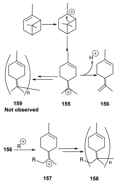
Scheme 44 Metal-based Lewis acid promoted cationic polymerization of α-pinene.
