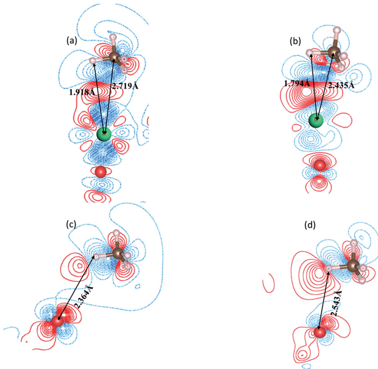
Fig. 3 2-D plots of the calculated electron density difference (EDD) for the \text{CH}_4 adsorption. (a) \text{C-H}\cdots\text{Ir} coplanar on \text{Ir}/\alpha\text{-Fe}_2\text{O}_3(110) surface, (b) \text{C-H}\cdots\text{Ir} coplanar on \text{Ir}/\alpha\text{-Fe}_2\text{O}_3(110)\text{-O}_\text{v} surface and (c) \text{C-H}\cdots\text{O} coplanar on \text{Ir}/\alpha\text{-Fe}_2\text{O}_3(110) surface and (d) \text{C-H}\cdots\text{O} coplanar on \text{Ir}/\alpha\text{-Fe}_2\text{O}_3(110)\text{-O}_\text{v} surface. The red and blue lines represent the increasing and decreasing electron densities, respectively. The isovalue is 0.002 \text{ ebohr}^{-3} .
