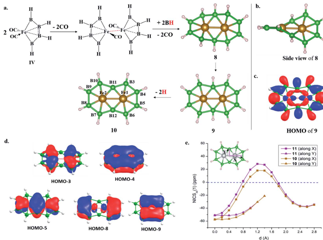
Fig. 2 (a) The design principle of \text{Fe}_2\text{@B}_{10}\text{H}_{10} ( 8 ) and \text{Fe}_2\text{@B}_{10}\text{H}_8 ( 10 ), starting from a B–B homocatenated complex ( IV , \text{R} = \text{H} ); planar \text{Fe}_2\text{@B}_{10}\text{H}_{10} ( 9 ) is not a minimum. (b) A side view of \text{Fe}_2\text{@B}_{10}\text{H}_{10} ( 8 ). (c) The HOMO of 9 . (d) The five \pi -MOs of 10 . (e) NICS zz (1) scan curves of 10 and 11 with the distance ( d ) increasing from the top of the ring center towards the periphery along X and Y directions.
