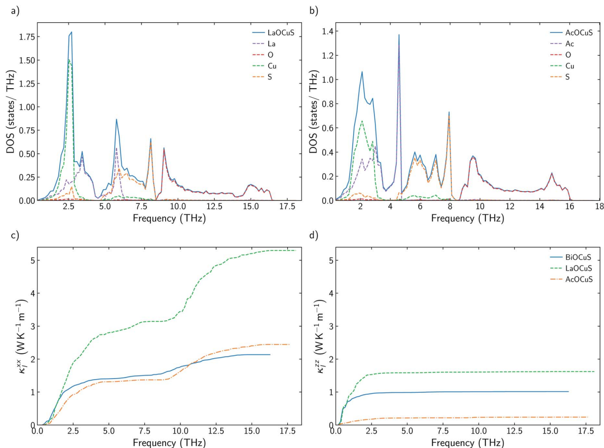
Fig. 3 (a and b) Total and projected phonon density of states, DOS, of LaOCuS and AcOCuS. (c and d) Cumulative \kappa_I^{xx} and \kappa_I^{zz} for BiOCuS, LaOCuS, and AcOCuS at 300 K.
