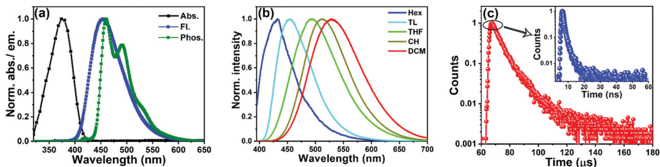
Fig. 2 (a) Normalized absorption, fluorescence ( \lambda_{ex} = 405 nm) and phosphorescence ( \lambda_{ex} = 405 nm) spectra of 3BPpy-pDTC in toluene (10 μM). (b) Normalized fluorescence ( \lambda_{ex} = 405 nm) spectra of 3BPpy-pDTC in solvents of varying polarity. Hex: hexane (0.009), TL: toluene (0.099), THF: tetrahydrofuran (0.207), CH: chloroform (0.259) and DCM: dichloromethane (0.309). The solvent polarity parameter ( E_T^N value) is mentioned in the parenthesis. (c) Emission decay profile ( \lambda_{ex} = 400 nm LED source) of 3BPpy-pDTC in degassed toluene at room temperature showing delayed fluorescence; inset: decay ( \lambda_{ex} = 410 nm diode laser source) at the nanosecond timescale indicating prompt fluorescence.
