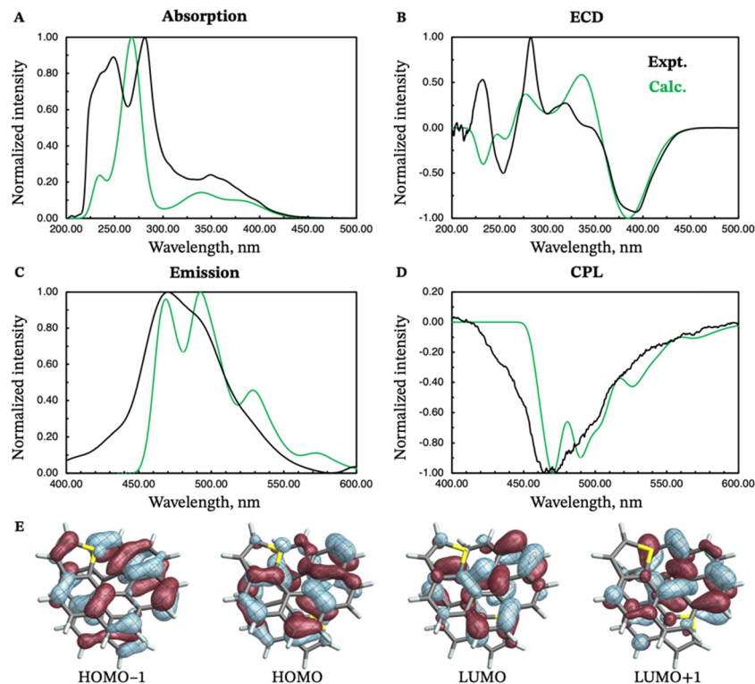
Fig. 6 Experimental (black curves) and calculated (green curves) absorption (panel A), ECD (panel B), emission (panel C) and CPL (panel D) spectra of (M)-endo-dithia[9]helicene 2 . Isosurfaces ( \pm 0.03 au) for the most relevant frontier molecular orbitals (HOMO-1, HOMO, LUMO, and LUMO+1) are shown in panel E. The calculated energies were shifted by -0.40 eV prior to conversion to wavelengths.
