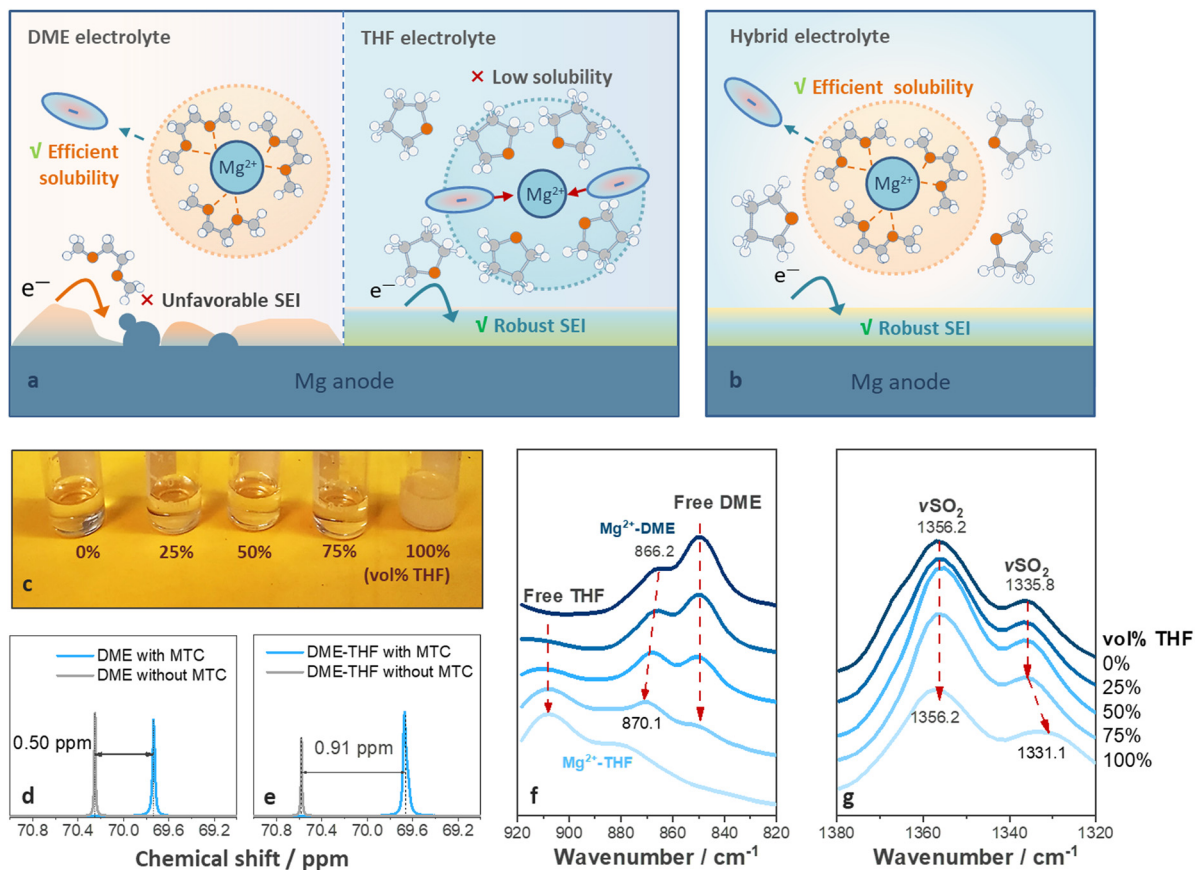
Fig. 1 Schematic illustration of structure of (a) single-solvent and (b) hybrid electrolytes. (c) Digital photographs of DME, DME-THF (25–75 vol% THF), and THF electrolytes. 13 C NMR spectra of methylene carbons in DME (d) without and (e) with THF (75 vol% THF). (f) and (g) Ex situ FT-IR spectra of DME, DME-THF (25–75 vol% THF), and THF electrolytes.
