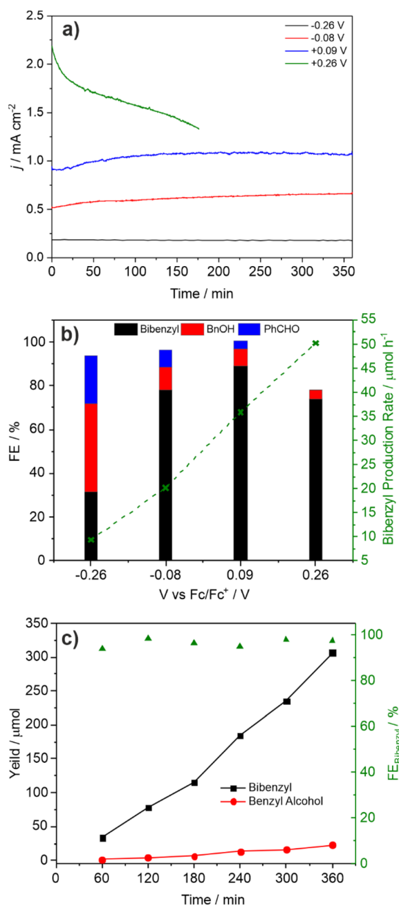
Fig. 3 (a) CPE of 1 \text{ M} PAA with 0.05 equiv. \text{Et}_3\text{N} at -0.26 (black), -0.08 (red), +0.09 (blue) and +0.26 V vs. \text{Fc}/\text{Fc}^+ ; (b) faradaic efficiencies for bibenzyl (black), benzyl alcohol (red) and benzaldehyde (blue) as a function of electrolysis potential; (c) time-dependent bibenzyl (black) and benzyl alcohol (red) formation at +0.09 V vs. \text{Fc}/\text{Fc}^+ of 1 \text{ M} PAA with 0.05 equiv. \text{Et}_3\text{N} . Overall faradaic efficiency for bibenzyl is given in green.
