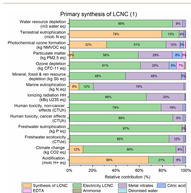
Fig. 3 Reference LCA results for the primary synthesis of (\text{La}_{0.9}\text{Ca}_{0.1})_2\text{Ni}_{0.75}\text{Cu}_{0.25}\text{O}_{4.6} (LCNC) visualised as respective relative impact contributions to each individual impact category from the main contribution categories ( e.g. , electricity). For absolute values, see Table 2 in section 2.3 (H: hydrogen, eq.: equivalent, CTUe: comparative toxic unit for ecosystems, P: phosphorus, CTUh: comparative toxic unit for human, HH: human health, U235: uranium 235, N: nitrogen, Sb: antimony, CFC-11: trichlorofluoromethane, PM: particulate matter, NMVOC: non-methane volatile organic compound).
