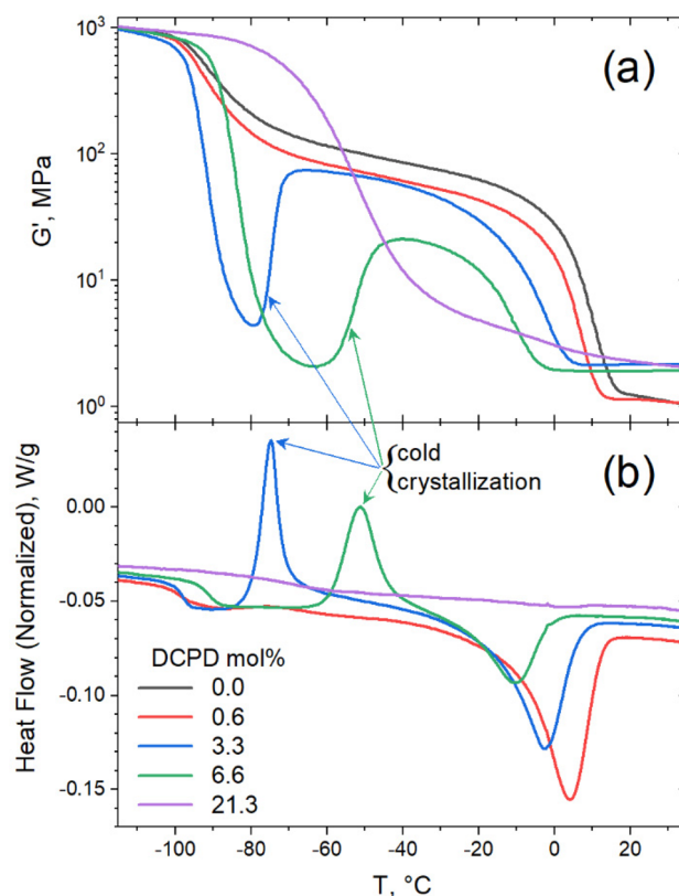
Fig. 5 Cold crystallization in moderate level DCPD content shown by (a) dynamic mechanical temperature sweep (monitoring G' ) and (b) DSC thermograms, after quench (-60 °C min -1 ) and with slow heat (2 °C min -1 ).
