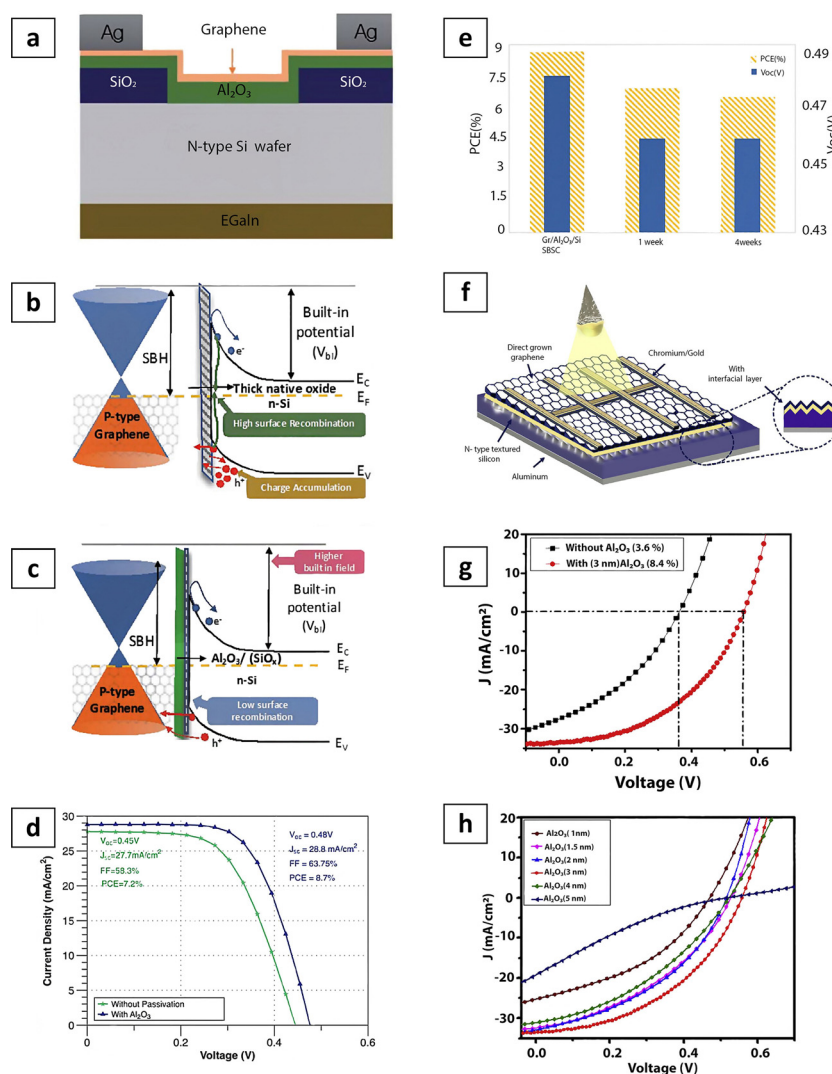
Fig. 5 (a) Schematic of Gr/ \text{Al}_2\text{O}_3 /Si device. (b) and (c) the energy band diagram of devices with and without \text{Al}_2\text{O}_3 layer. (d) J-V characteristics of devices. (e) Variations of PCE and V_{oc} of Gr/Si with \text{Al}_2\text{O}_3 interfacial layer by time. Reproduced from ref. 106, with permission from the Royal Society of Chemistry. (f) Metal-insulator-semiconductor Schottky solar cells by \text{Al}_2\text{O}_3 layer. (g) J-V characteristics of the devices under illumination with and without an \text{Al}_2\text{O}_3 layer. (h) Comparison of J-V for different thicknesses of the \text{Al}_2\text{O}_3 layer. Reproduced from ref. 108, with permission from Elsevier.
