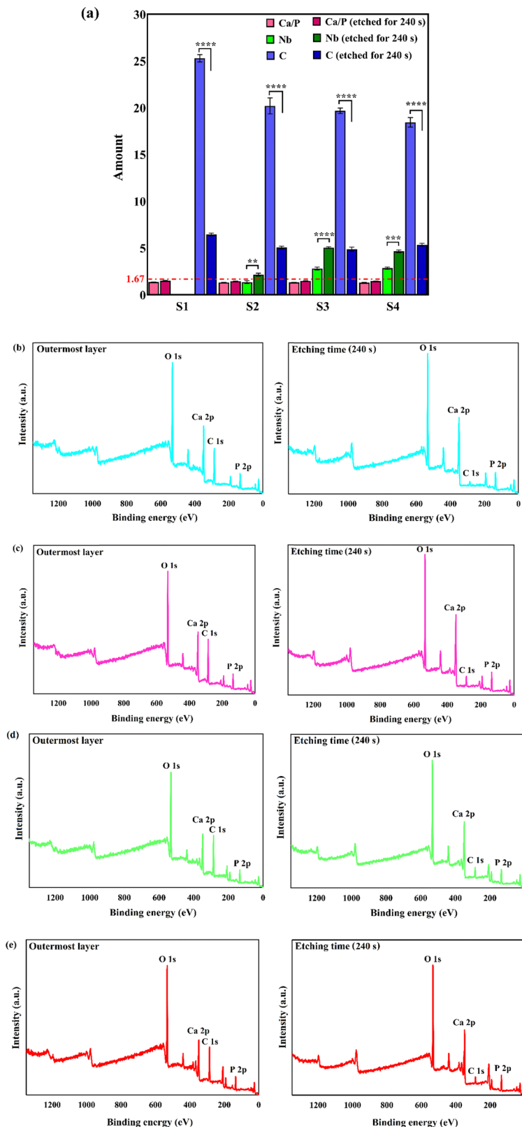
Fig. 6 (a) The XPS-derived data, including Ca/P ratio and atomic percent of Nb and C elements ( **p = 0.0013 , ***p = 0.0001 , and ****p < 0.0001 ); and XPS survey spectra of the outermost and subsurface layers: (b) S1, (c) S2, (d) S3, and (e) S4.
