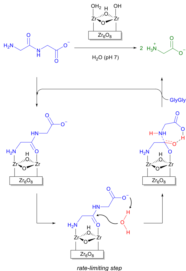
Scheme 1 General mechanism of peptide bond hydrolysis at the \text{Zr}_6\text{O}_8 cluster nodes of Zr-MOFs.
