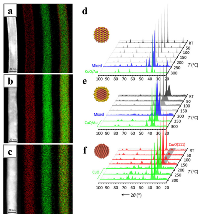
Fig. 21 (a–c) HAADF-STEM images and EDS elemental mappings of (a) pristine Cu@Au core-shell nanowire (b) an intermediate obtained after annealing the Cu@Au nanowires at 200 °C and (c) \text{CuAu} alloy nanowires obtained after annealing the Cu@Au nanowires at 320 °C. XRD patterns of (d) \text{Cu}_3\text{Au} , (e) Cu@Au core-shell prepared at 140 °C and (f) Cu nanowires after annealing in air for 1 hour at elevated temperatures. Reprinted with permission from ref. 162. Copyright 2020 from Springer Nature.
