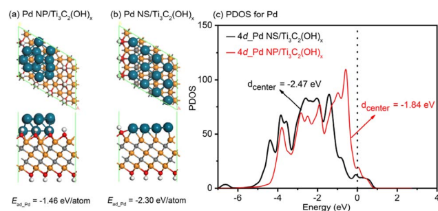
Fig. 6 The relaxed atomic structures of the (a) Pd NP/ \text{Ti}_3\text{C}_2(\text{OH})_x and (b) Pd NS/ \text{Ti}_3\text{C}_2(\text{OH})_x models, where the gray, red, white, orange, and blue balls represent C, O, H, Ti, and Pd atoms, respectively. (c) The d-PDOS plots of the different Pd nanostructures in the Pd NP/ \text{Ti}_3\text{C}_2(\text{OH})_x and Pd NS/ \text{Ti}_3\text{C}_2(\text{OH})_x models.
