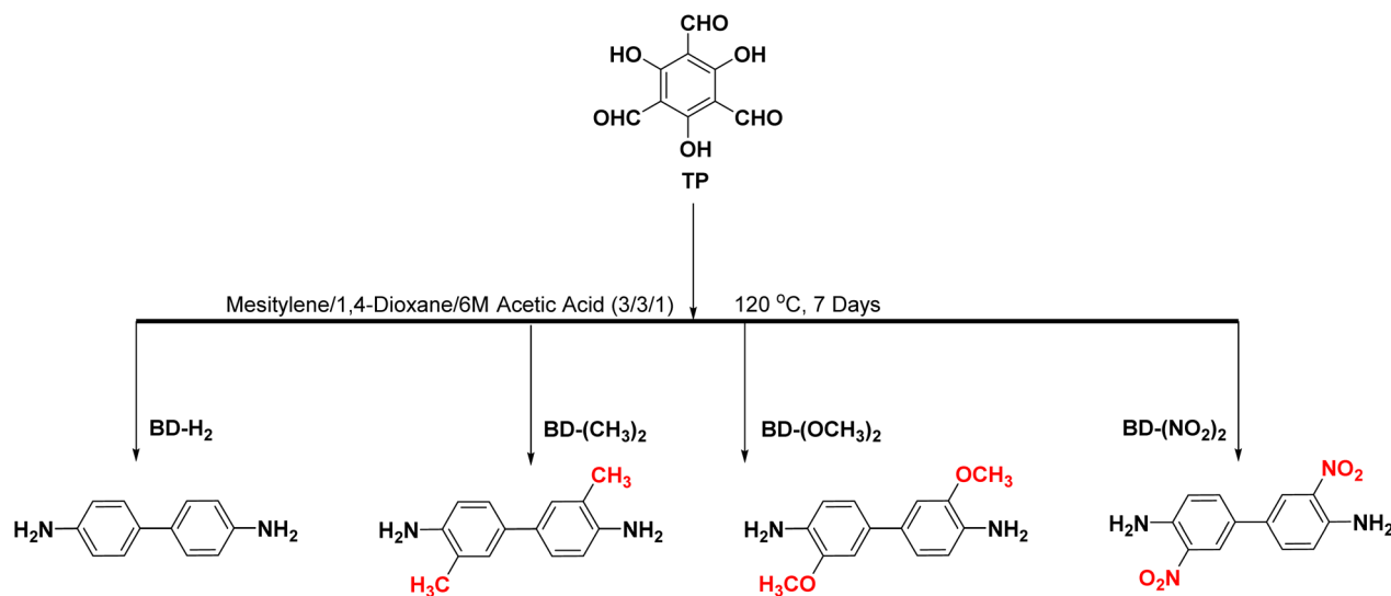
Fig. 8 Schematic diagram of the synthetic path for TpBD-X [X = \text{-H}_2 , \text{-(CH}_3)_2 , \text{-(OCH}_3)_2 , and \text{-(NO}_2)_2 ].
