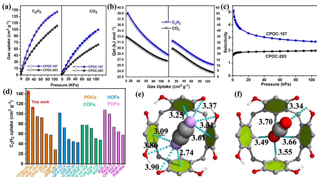
Fig. 3 (a) C 2 H 2 and CO 2 sorption isotherms at 298 K; (b) Q_{st} values of C 2 H 2 and CO 2 ; (c) the C 2 H 2 /CO 2 IAST selectivity; (d) comparison of C 2 H 2 uptakes with different top-performed POM adsorbents under ambient conditions; (e) C 2 H 2 and (f) CO 2 adsorption sites in CPOC-107 performed in order to understand its C 2 H 2 /CO 2 separation mechanism. Carbon is gray, oxygen red, and hydrogen lavender. Dashed bonds highlight H...π and H...O interactions.
