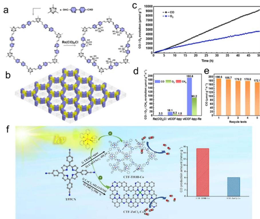
Fig. 17 (a) The synthesis of viCOF-bpy and viCOF-bpy-Re. (b) Diagram of the alternating arrangement of bipyridine and triazine ring units. (c) Time-dependent \text{CO} and \text{O}_2 production performance of viCOF-bpy-Re. (d) Photocatalytic \text{CO}_2 reduction performance of the Re-complex, viCOF-bpy, and viCOF-bpy-Re. (e) Stability tests of viCOF-bpy-Re. Reproduced with permission from ref. 208. Copyright 2023, John Wiley and Sons. (f) Porphyrin-based CTFs for photocatalytic \text{CO}_2 reduction. Reproduced with permission from ref. 209. Copyright 2023, Elsevier.
