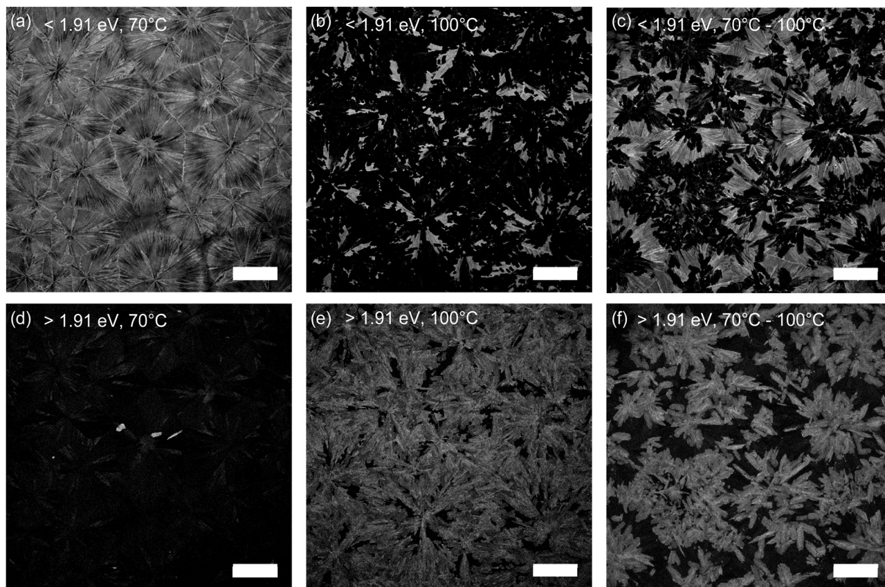
Fig. 4 Confocal photoluminescence micrographs in the range < 1.91 eV (a–c) and > 1.91 eV (d–f) for OBESnI 4 thin films processed at 70 °C, 100 °C, and 70–100 °C. Scale bar is 100 μm.
