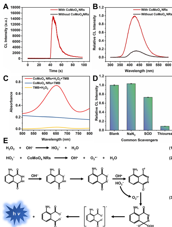
Fig. 9 (A) CL intensity–time curves and (B) CL spectra of the luminol/ \text{H}_2\text{O}_2 system in the absence and presence of \text{CoMoO}_4 NRs. CBS pH 11.0, [luminol]: 1\text{ }\mu\text{M} ; [ \text{H}_2\text{O}_2 ]: 50\text{ }\mu\text{M} ; [ \text{CoMoO}_4 NRs]: 20\text{ }\mu\text{g mL}^{-1} . (C) UV-vis absorption spectra of TMB/ \text{H}_2\text{O}_2 , \text{CoMoO}_4 NRs/ \text{H}_2\text{O}_2 , and \text{CoMoO}_4 NRs/ \text{H}_2\text{O}_2 /TMB systems. NaAc/HAc buffer solution pH 4.0, [TMB]: 0.1\text{ mM} ; [ \text{H}_2\text{O}_2 ]: 25\text{ mM} ; [ \text{CoMoO}_4 NRs]: 50\text{ }\mu\text{g mL}^{-1} . (D) Relative CL intensity of luminol/ \text{H}_2\text{O}_2 / \text{CoMoO}_4 NRs with common radical scavengers including 1\text{ mM Na}_2\text{S}_2\text{O}_3 , 5\text{ }\mu\text{g mL}^{-1} SOD, and 1.0\text{ mM thiourea} . CBS pH 11.0; [luminol]: 1\text{ }\mu\text{M} ; [ \text{H}_2\text{O}_2 ]: 50\text{ }\mu\text{M} ; [ \text{CoMoO}_4 NRs]: 20\text{ }\mu\text{g mL}^{-1} . (E) CL mechanism of the luminol/ \text{H}_2\text{O}_2 / \text{CoMoO}_4 NR system. Reprinted with permission from ref. 61, Copyright 2024 American Chemical Society.
