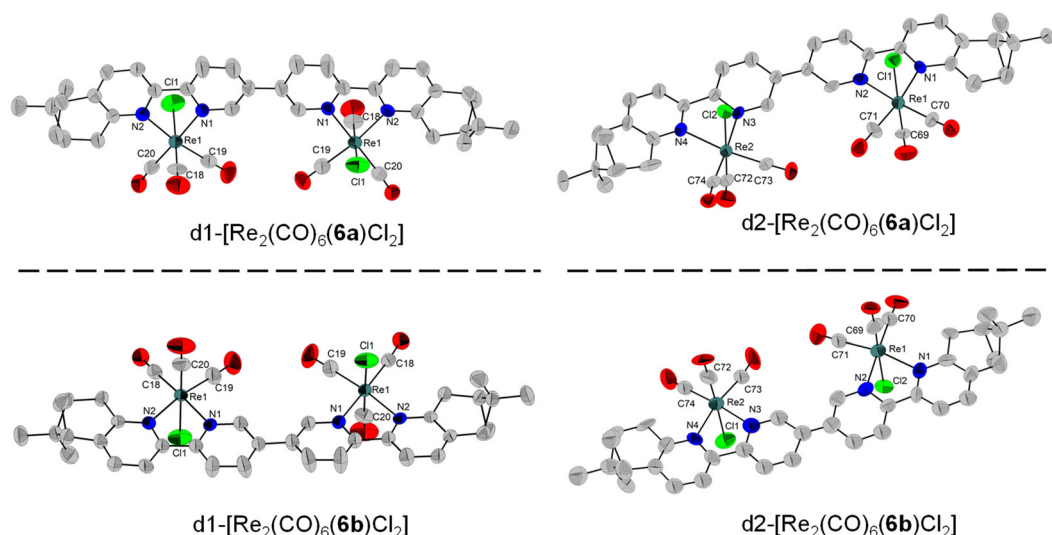
Fig. 5 Single-crystal X-ray diffraction structures of the four stereoisomers obtained with the ligands 6a and 6b , depicting the enantiomeric pairs obtained. The H atoms were removed for clarity.
