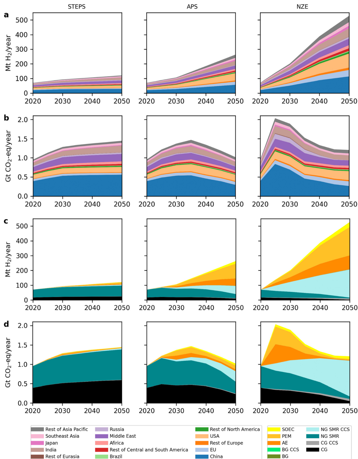
Fig. 4 In three scenarios, the global H 2 production and annual GHG emissions in 15 regions. (c) and (d) Show H 2 production volumes and annual GHG emissions of nine technologies. CG = coal gasification, NG SMR = steam methane reforming of natural gas, BG = biomass gasification, CCS = carbon capture and storage, AE = alkaline electrolyzer, PEM = proton exchange membrane electrolyzer, and SOEC = solid oxide electrolysis cell. The water electrolysis is coupled with grid electricity. Although BG CCS has negative emissions, its final contribution is very small because of its limited adoption.
