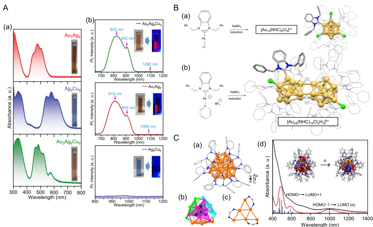
Fig. 8 (A) (a) Absorbance spectra of [Au 7 Ag 8 (C≡C t Bu) 12 ] + , [Ag 9 Cu 6 (C 6 H 9 ) 12 ] + and [Au 2 Ag 8 Cu 5 (C≡C t Bu) 12 ] + . (b) The emission spectra of [Au 7 Ag 8 (C≡C t Bu) 12 ] + ( \lambda_{\text{ex}} = 482 nm), [Ag 9 Cu 6 (C 6 H 9 ) 12 ] + ( \lambda_{\text{ex}} = 580 nm) and [Au 2 Ag 8 Cu 5 (C≡C t Bu) 12 ] + ( \lambda_{\text{ex}} = 490 nm) in dichloromethane. Inset: photographs of the three NCs in dichloromethane under room light (left) and 365 nm UV-light (right), respectively. (B) Production of different NHC-stabilized Au clusters depending on the ancillary ligand (halide or pyridine). (a) Use of halide ligands gives typical Au 13 clusters ([Au 13 (NHC) 9 Cl 3 ] 2+ ), while (b) labile ancillary ligand leads to hydride bridged Au 24 clusters ([Au 24 (NHC) 14 Cl 2 H 3 ] 3+ ). (C) (a) The overall structure of [Au 28 (Ph-form) 12 ] 2+ . (b) The T symmetrical Au 28 kernel with concentric tetrahedral Au 4 core (black) and truncated tetrahedron Au 24 shell divided into four {111} faces. (c) The bridge mode of formamidinate ligands; all Ph rings are omitted for clarity. (d) The experimental (black) and simulated (red) absorption spectra of Au 28 . (Inset) The NTO picture of the first absorption peak. (A) is reproduced with permission from ref. 245. Copyright 2022 Royal Society of Chemistry. (B) is reproduced with permission from ref. 249. Copyright 2022 American Chemical Society. (C) is reproduced with permission from ref. 250. Copyright 2021 Wiley-VCH GmbH.
