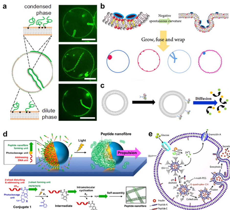
Fig. 11 Proteins and peptides for actuating lipid membranes. a, GUV deformation triggered by phase separation of FUS LC adhered on the lipid membrane. Scale bars: 10 μm. 279 b, GUV deformation triggered by de novo peptides. 285 c, Propulsion of ATPase-coated GUVs. 286 d, Light-induced propulsion of a phase-separated GUVs driven by local peptide nanofibre growth (top) and the photocleavage reaction of a DNA-peptide conjugate (bottom). 289 e, Illustration of the biochemical process inside OLVs. Vesicle fusion is triggered by the interaction between peptide K and peptide E. 364 Figures reproduced with permission from: a, ref. 279, copyright 2021, National Academy of Sciences; b, ref. 285, copyright 2018, American Chemical Society; c, ref. 286, copyright 2019, American Chemical Society; d, ref. 289, copyright 2018, Nature Publishing Group; e, ref. 364, copyright 2021, Royal Chemical Society.
