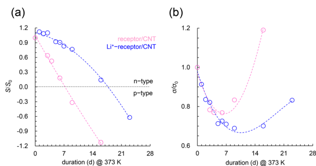
Fig. 4 Stability of unencapsulated receptor/CNT and Li + -receptor/CNT in air at 373 K. (a) n-type seebeck coefficient ( S/S_0 ), and (b) electrical conductivity ( \sigma/\sigma_0 ) over duration.
