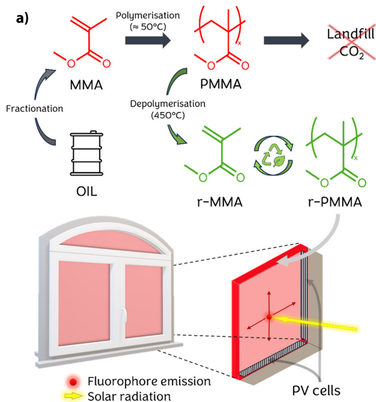
Fig. 1 (a) Representation of the luminescent solar concentrator (LSC) technology installed in a window. The LSC host material is PMMA obtained from chemical recycling (marked in green), which replaces the standard production from oil (in grey); (b) a prototype of multi-fluorophore LSC systems installed on a bus shelter; and (c) an LSC coupled to a silicon photovoltaic cell under direct solar irradiation.
