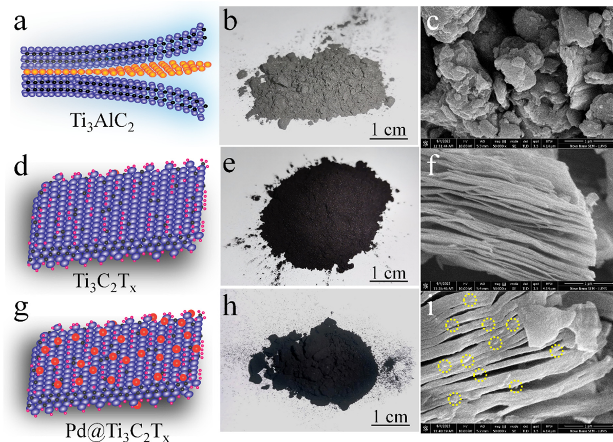
Fig. 3 (a) Schematic illustration, (b) digital photograph, and (c) SEM image of MAX ( \text{Ti}_3\text{AlC}_2 ). (d) Schematic illustration, (e) digital photograph, (f) SEM image of MXene ( \text{Ti}_3\text{C}_2\text{T}_x ). (g) Schematic illustration, (h) digital photograph, and (i) SEM image of Pd@MXene ( \text{Pd@Ti}_3\text{C}_2\text{T}_x ).
