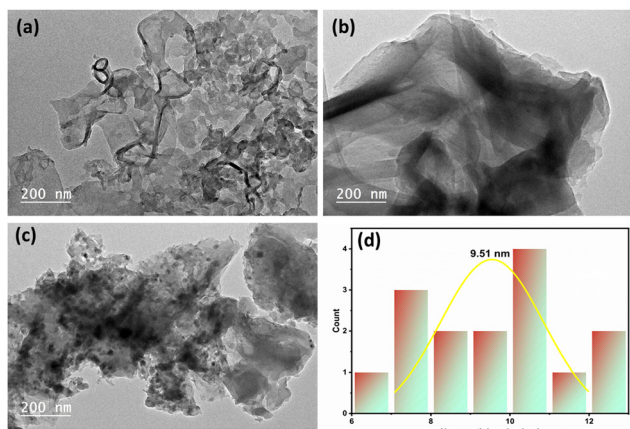
Fig. 6 TEM analysis of (a) g-C 3 N 4 , (b) CoCN-NaBH 4 , and (c) CoCN-H 2 . (d) NP size distribution histogram of CoCN-H 2 .
