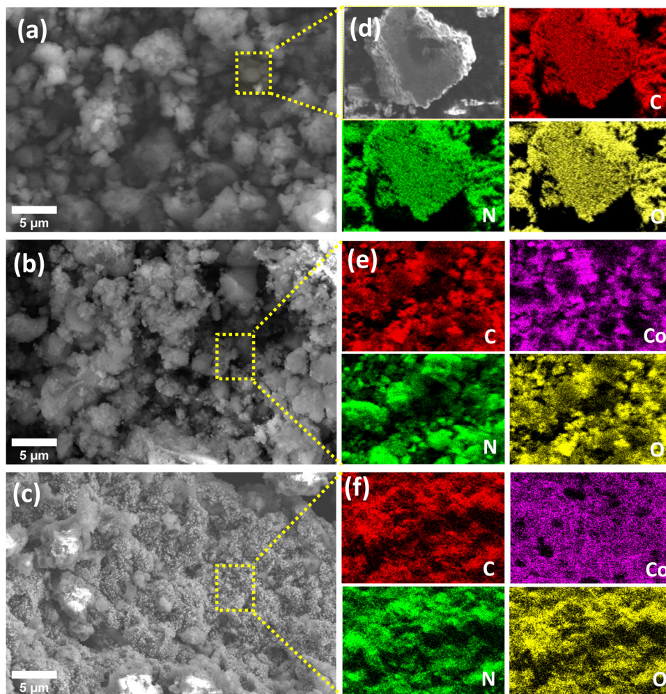
Fig. 5 SEM micrographs and EDS mapping of (a) and (d) g-C 3 N 4 , (b) and (e) CoCN-NaBH 4 , and (c) and (f) CoCN-H 2 .
