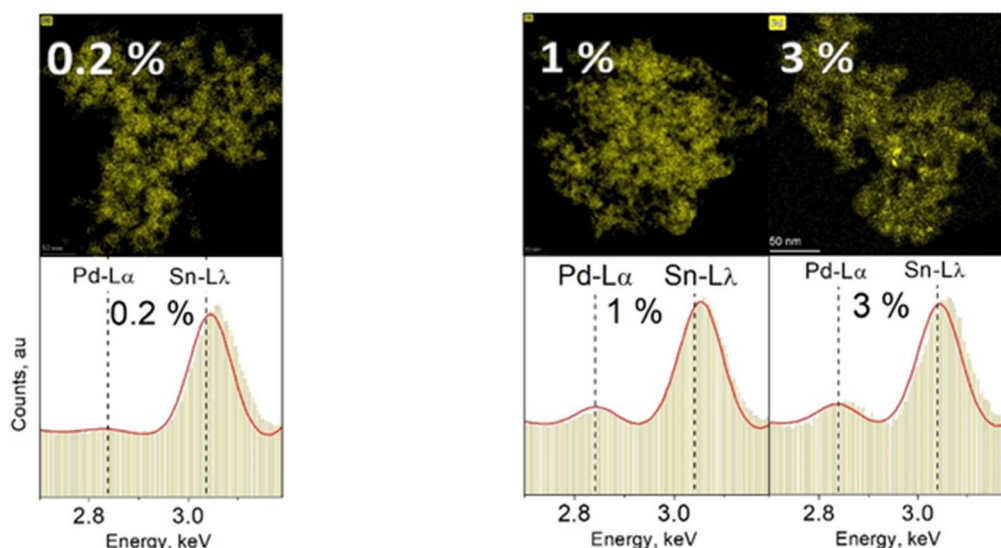
Fig. 3 (a) Top panel: Pd elemental maps of annealed \text{SnO}_2 doped with Pd contents of 0, 0.2, 0.5, 1 & 3 mol% and made at C = 0.5 M, P/D = 5/5 . Bottom panel: EDXS spectra corresponding to the image area above. All images were recorded at the same imaging conditions (450 kx magnification, beam current of 8 nA, 10 frames at 50 \mu\text{s} dwell time). As the content of Pd increases, more and larger Pd-rich (bright) spots are visible. (b) Top panel: Pd elemental maps of \text{SnO}_2 containing originally 0.2, 1 & 3 mol% Pd after undergoing leaching with \text{HNO}_3 . Only in the 3 mol% sample some Pd-rich spots are visible. The bottom panel: EDXS spectra corresponding to the image area above. Clearly, the amount of Pd in relation to Sn has decreased compared to these samples before leaching and corresponds to the embedded Pd into \text{SnO}_2 .
