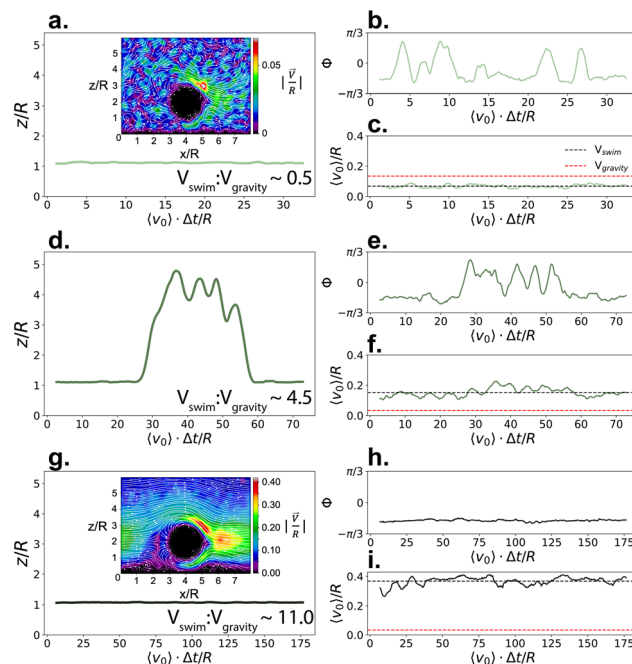
Fig. 3 Dynamics of CB microswimmers, simulated to reproduce the properties of the chemical active colloids studied in ref. 20. z/R refers to the height that a microswimmer reaches above the substrate with respect to its radius R (a, d, and g). \phi is the azimuthal angle of the microswimmer (b, e, and h) as defined in Fig. 1, and v_0 is the time-series of the microswimmer's instantaneous velocity (c, f, and i, with V_{\text{swim}} = \langle v_0 \rangle / R ). The insets in (a) and (g) show the solvent velocity flow fields around the (fixed) microswimmer at the different self-propulsion forces. Here, we progressively increase the swimming to sedimentation velocity ( V_{\text{swim}} : V_{\text{gravity}} ) from top to bottom to qualitatively map onto the different systems studied by Carrasco-Fadanelli and Buttinoni. The first two cases (a–c and d–f) are in good agreement with the findings presented in ref. 20, while the final case (g–i) recaptures the typical dynamics observed for chemical active colloids, where phoretic particles are essentially confined to 2-D (also see Fig. 2b).
