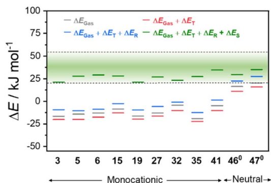
Fig. 7 Relative spin-state energy of VT monocationic [\text{Co}(\text{X}^{\text{diox}})(\text{N}_4\text{-L})]^+ and neutral [\text{Co}(3,5\text{-dbdiox})(3,5\text{-dbsq})(\text{N}_2\text{L})] families illustrating the cumulative effects from the gas phase ( \Delta E_{\text{Gas}} ) (grey); relative gas phase energy with thermal effects ( \Delta E_{\text{Gas}} + \Delta E_{\text{T}} ) (red); relative gas phase energy with thermal and relativistic effects ( \Delta E_{\text{Gas}} + \Delta E_{\text{T}} + \Delta E_{\text{R}} ) (blue); relative gas phase energy with thermal, relativistic and solvent effects in MeCN ( \Delta E_{\text{Gas}} + \Delta E_{\text{T}} + \Delta E_{\text{R}} + \Delta E_{\text{S}} ) (green). (The green region illustrates the experimental VT energy region in solution).
