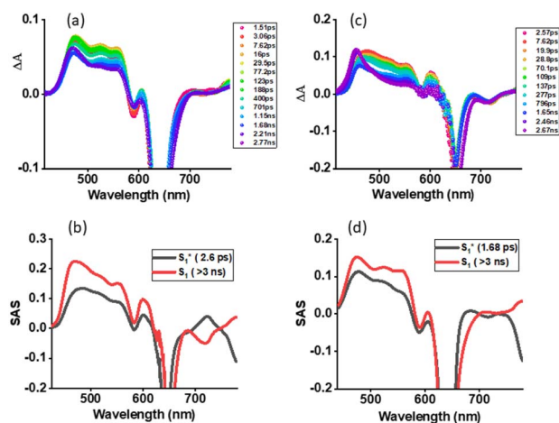
Fig. 6 Femtosecond transient absorption spectra at the indicated delay times of (a) 1 and (c) 2 in toluene ( \lambda_{\text{ex}} = 648 nm). Species associated spectrum from Glotaran analysis is shown beneath for each spectrum.
