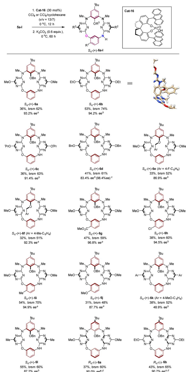
Scheme 3 Catalytic enantioselective synthesis of inherently chiral N 3 ,O-calix[2]arene[2]triazines 6a–l and the X-ray molecular structure of S 1C - 6b . a Reaction was performed in a mixture of CCl 4 and cyclohexane (v/v = 13/7). b Reaction was carried out in pure CCl 4 . c The ee value was obtained after recrystallization. d Enantiomer of Cat-16 was used as the chiral catalyst.
