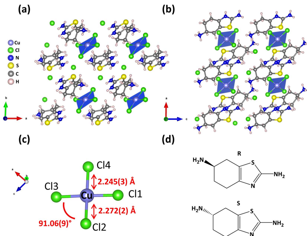
Fig. 1 Part of the crystal structure of (R-THBTD) 2 CuCl 6 viewed along the (a) c -axis and (b) b -axis, respectively. (c) Representation of the square planar geometry of the [CuCl 4 ] 2− moieties along with two representative Cu–Cl bond lengths and one Cl–Cu–Cl angle. (d) The molecular structures of the chiral ligands S-THBTD and R-THBTD.
