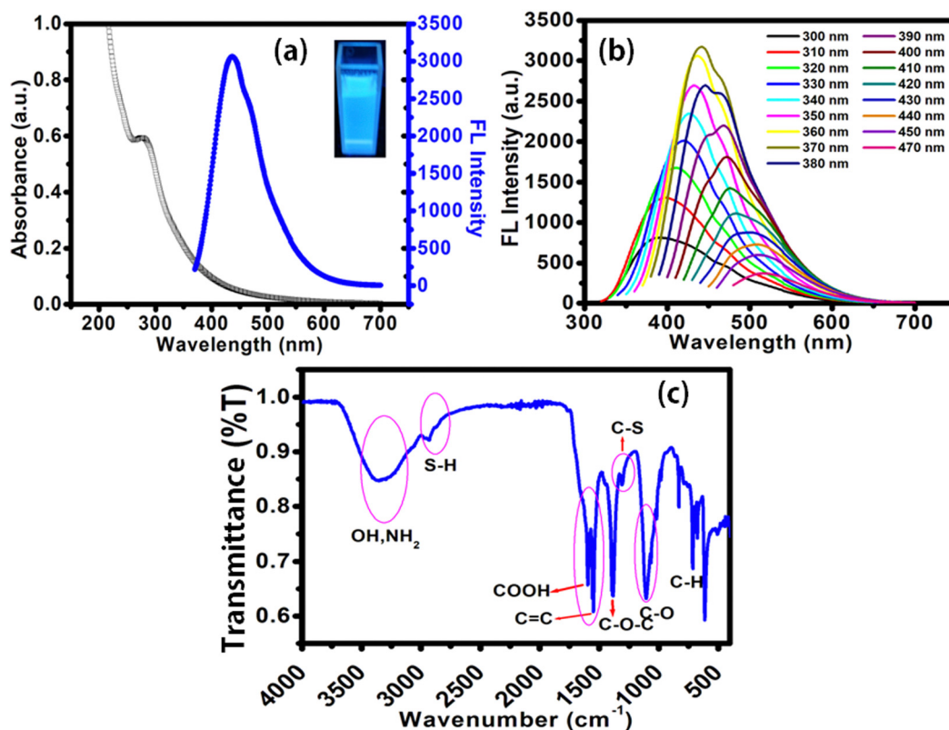
Fig. 1 (a) Absorption and FL spectra of OGDs excited at 360 nm. Inset: Strong blue FL of OCD solution observed by the naked eyes under 365 nm UV lamp illumination. (b) FL spectra of OGDs excited at different wavelengths ranging from 300 nm to 470 nm and (c) FT-IR spectra of OGDs.
