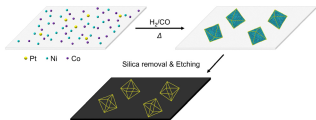
Scheme 1 Schematic illustration of the PtNiCo skeleton synthesis. Metal precursors supported on fumed silica undergo thermal annealing in a \text{H}_2/\text{CO} atmosphere, forming octahedral NPs. Subsequent HF etching removes silica and selectively leaches Ni and Co, forming an octahedral skeleton.
