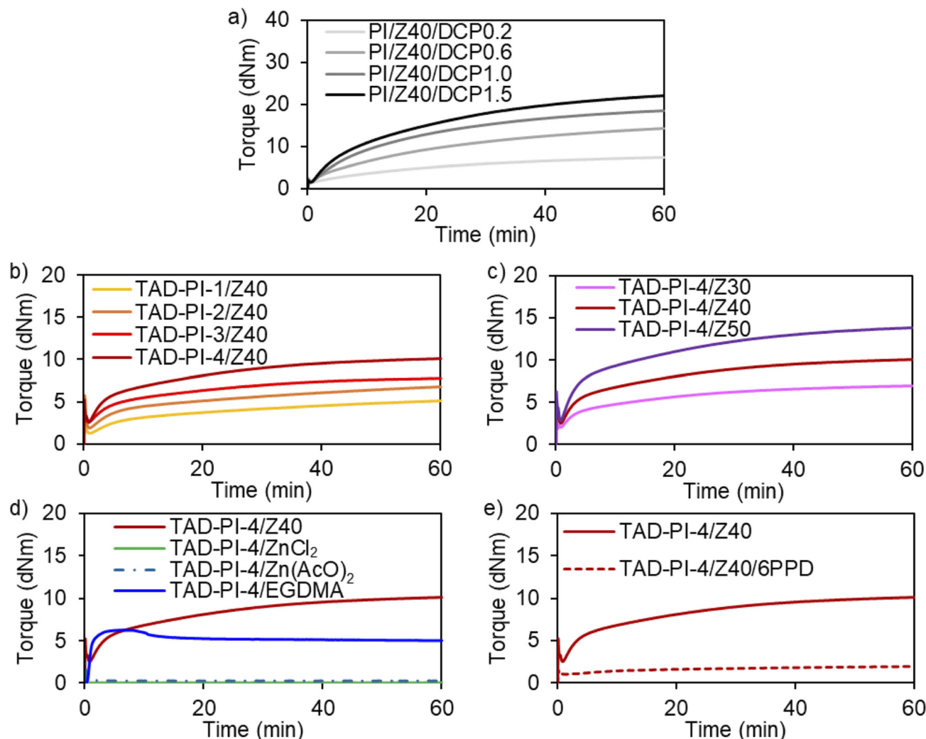
Fig. 4 Elastic-torque curves of rubber composites measured using a moving die rheometer at 145 °C: (a) control samples (PI/Z40/DCP), (b) effect of the amount of bound TAD in the PIs, (c) effect of the ZDMA content, (d) results for TAD-PI-4 with various types of chemicals and (e) the effect of the radical-trapping agent 6PPD.
