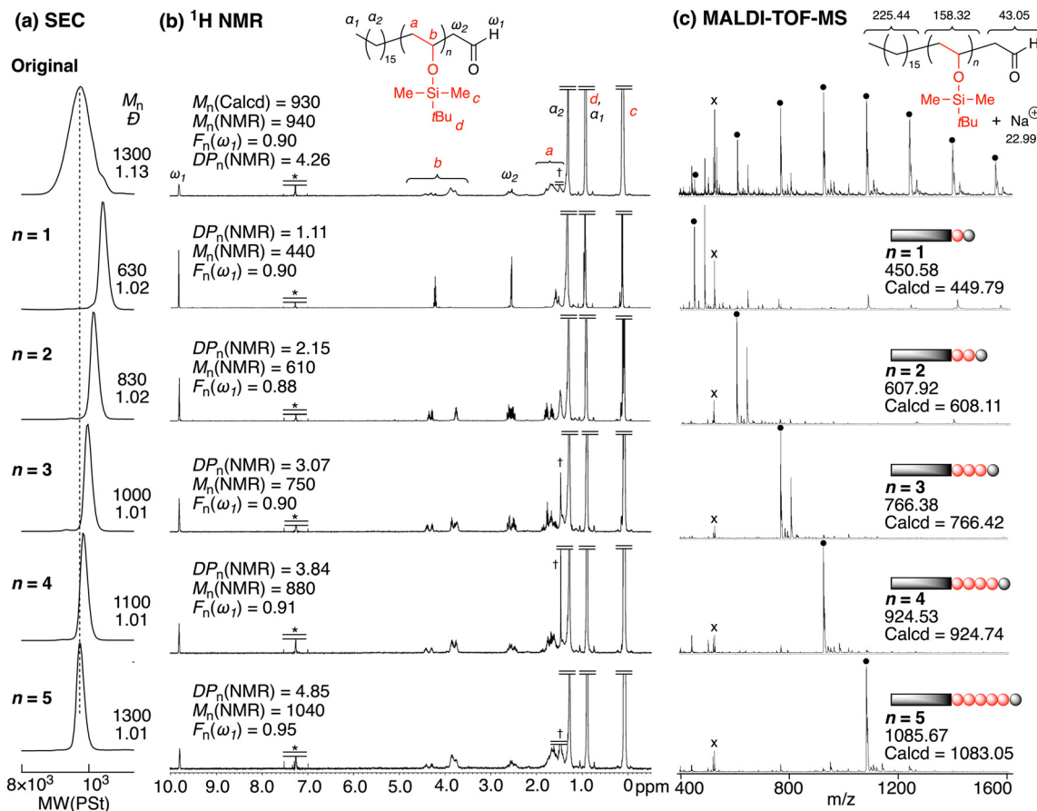
Fig. 3 SEC (a), ^1\text{H} NMR (b), and MALDI-TOF-MS (c) spectra of monodisperse oligo(TBSVE) fractionated by preparative recycling SEC. ^*\text{CHCl}_3 and ^\dagger\text{water} in (b). The peaks marked with "x" in (c) are derived from trans -2-[3-(4- tert -butylphenyl)-2-methyl-2-propenyldiene]malononitrile (DCTB) as the ionizing matrix.
