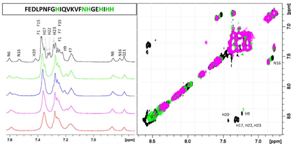
Fig. 2 Aromatic regions of 1D ^1\text{H} and 2D ^1\text{H} - ^1\text{H} TOCSY spectra of PvHct 0.5 mM, SDS- \text{d}_{26} 40 mM, pH 7.4 T 298 K in absence (black) and in presence of 0.2 (green), 0.4 (blue), 0.6 (magenta) and 0.8 (red) zinc(II) equivalents. The most affected residues of the peptide sequence are shown in green.
