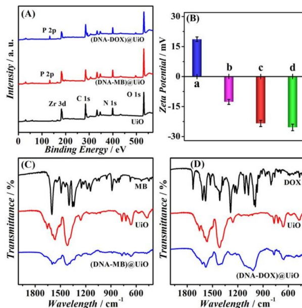
Fig. 2 (A) XPS survey spectra of UiO, (DNA-MB)/UiO, and (DNA-DOX)/UiO. (B) Zeta potential of UiO (a, blue), (DNA-MB)/UiO (b, magenta), (DNA-DOX)/UiO (c, red), and (DNA-DOX)/UiO (d, green). FT-IR spectra of (C) (DNA-MB)/UiO compared with MB and UiO, and (D) (DNA-DOX)/UiO compared with DOX and UiO. Error bar: standard deviation (SD) and the number of measurements ( n ): 3.
