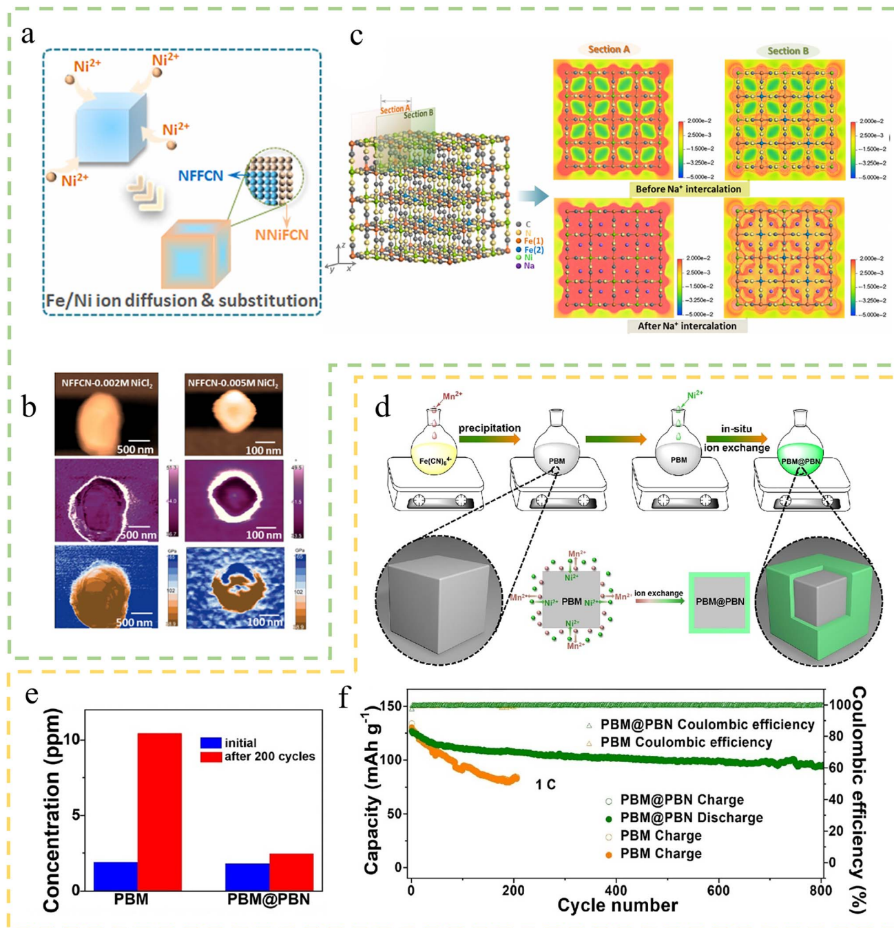
Fig. 14 (a) Schematic illustrating the preparation of core-shell NNiFCN/NFFCN. (b) AFM topography images, phase images, and stiffness tomography images of NFFCN-0.002 M \text{NiCl}_2 and NFFCN-0.005 M \text{NiCl}_2 (from up to down). (c) Electrostatic potential of NFFCN before and after \text{Na}^+ intercalation. 116 Copyright 2021, Springer Nature. (d) Schematic illustration of the synthesis process of the PBM@PBN sample. (e) Measurement of Mn dissolution in the electrolyte after a long-term cycle. (f) Cycling performance of PBM@PBN and PBM at 1C. 117 Copyright 2021, Elsevier.
