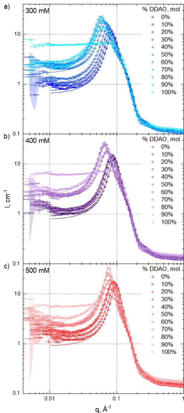
Fig. 3 Radially-averaged (1D) SANS scattering profiles for (a) 300 mM, (b) 400 mM, and (c) 500 mM isopleths, of fixed overall surfactant concentration, with varying SDS:DDAO ratio. Open circles ( \circ ) show data points and the solid lines are model fits using a core-shell form factor, P(q) , and Hayter-MSA structure factor, S(q) (except for 100% DDAO, for which a hard sphere structure factor was used).
