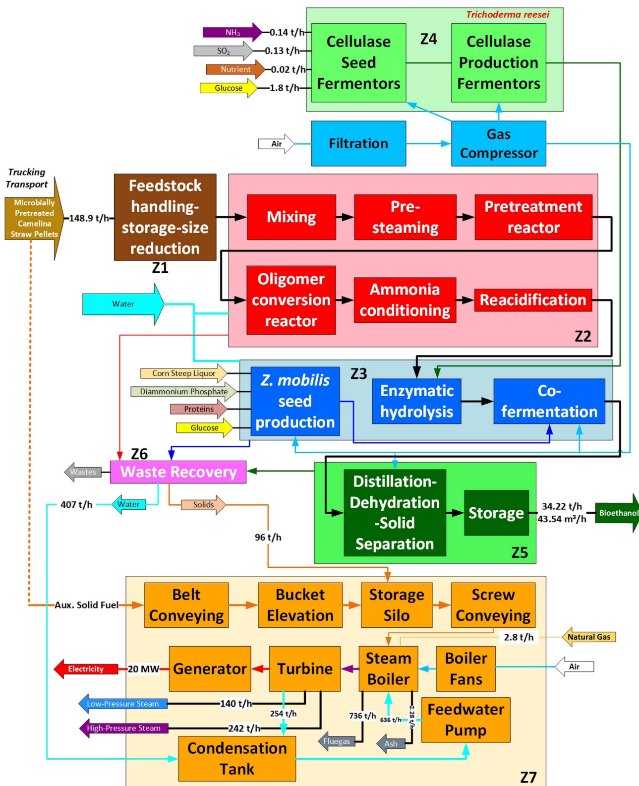
Fig. 4 Simplified block diagram of the modeled cellulosic ethanol production process using microbially pretreated cameline straw pellets as feedstock (Ethanol Plant A): farmer participation rate = 10%, pellet feedstock capacity = 148.90 t per h (note: green block: enzyme production, brown block: feedstock handling and storage, red block: pretreatment, blue block: enzymatic hydrolysis and fermentation, dark green block: product recovery, violet block: waste recovery, and orange block: co-generation plant).
