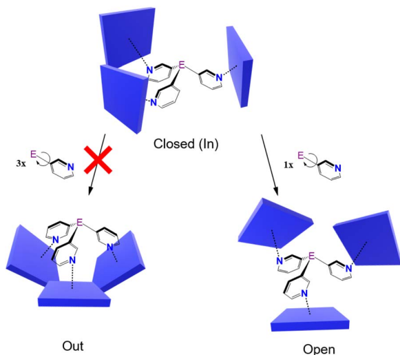
Fig. 3 Possible conformations of capsules of the type [(E(3\text{-py})_3)_3] \cdot (\text{ZnTPP})_3 .
