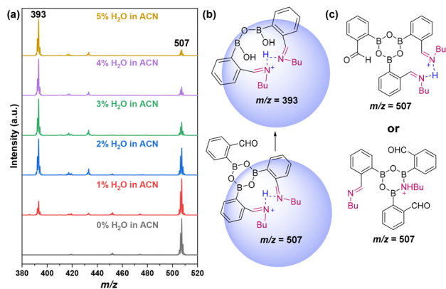
Fig. 3 (a) Positive mode nESI mass spectra of the products of reaction between butylamine and 2-FPBA using different ratios of \text{H}_2\text{O}:\text{ACN} in microdroplets. Here, water was added in specially dried ACN (see ESI,† Section 1.2). (b) Addition of water to the spray solvent gives the hydrolysis product, observed at m/z 393. (c) Isomeric chemical structures corresponding to m/z 507 are shown.
