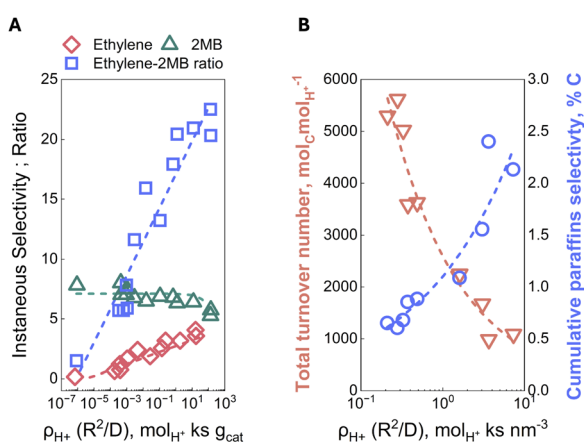
Fig. 5 (A) Instantaneous ethylene and 2MB (2-methylbutane, 2-methyl-2-butene) selectivity, ethylene-to-2MB ratio versus \frac{\rho_{H^+} R^2}{D} for DME conversion over HZSM-5 of varying crystallite size and Si/Al ratio at 623 K. (B) Total turnover number (left axis) and cumulative paraffins selectivity (right axis) for methanol conversion on HSAPO-34 at 673 K, 16 kPa methanol pressure. Adapted with permission from Bhan and coworkers. 59 Copyright J. Catal. 2023.
